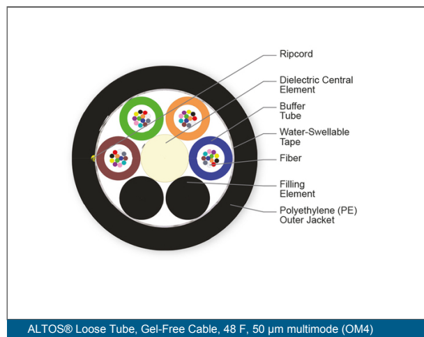
ALTOS® Loose Tube, Gel-Free Cable, 48 F, 50 µm multimode (OM4)
