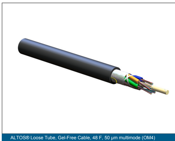
ALTOS® Loose Tube, Gel-Free Cable, 48 F, 50 µm multimode (OM4)
